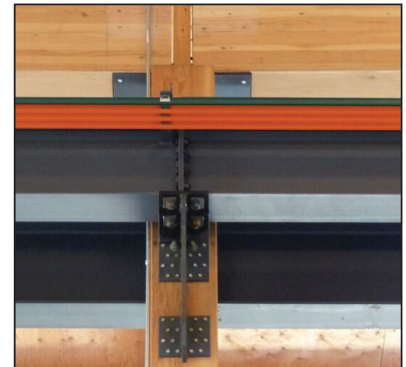
Fig. 4.11: Column-to-beam connection at gantry crane
