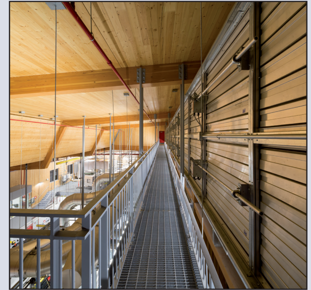
Fig. 3.8: The sloping roof also features structural CLT panels
