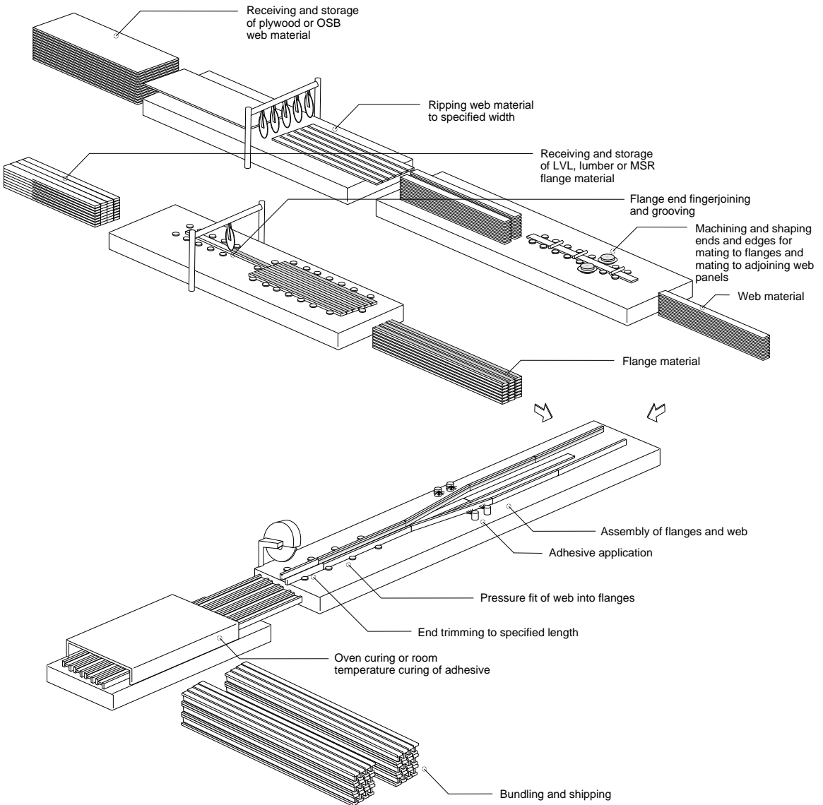
Figure 3.21 Manufacture of Prefabricated Wood I-Joists
