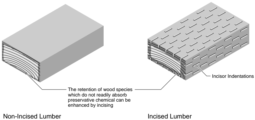
Figure 9.9 Cross Section of Preservative Treated Lumber
