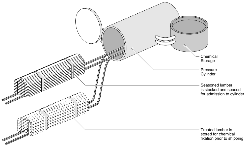
Figure 9.8 Manufacture of Pressure- Treated Wood
