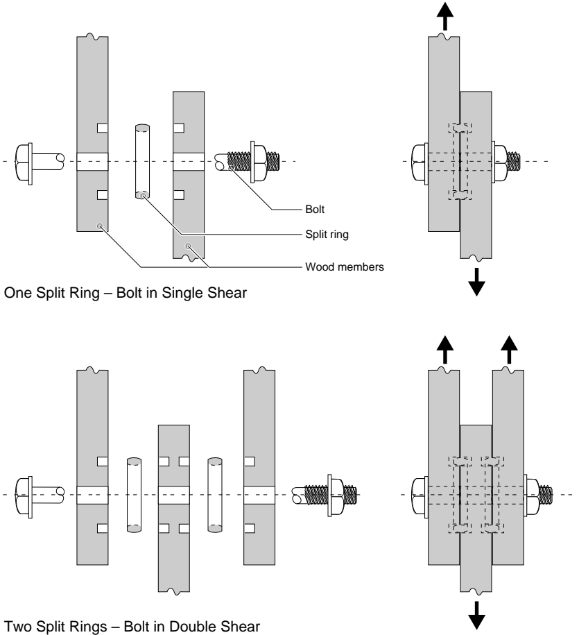
Split Ring Connector (Available in 63mm (2-1/2") and 100mm (4") diameters)
