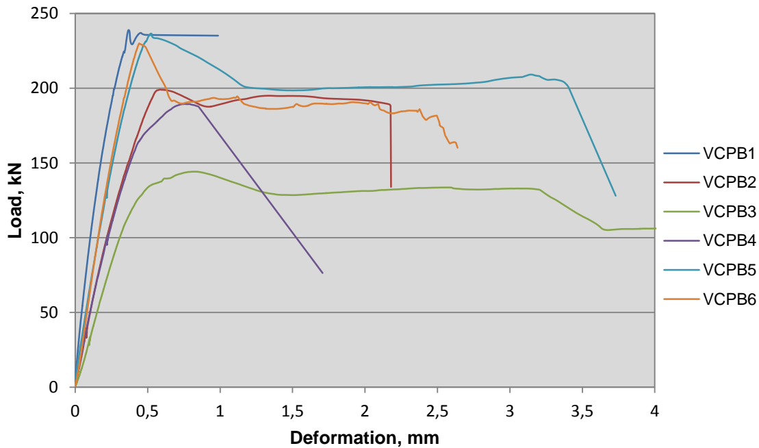
Figure 5. Load-deformation curves for all specimens of Series VCPB
