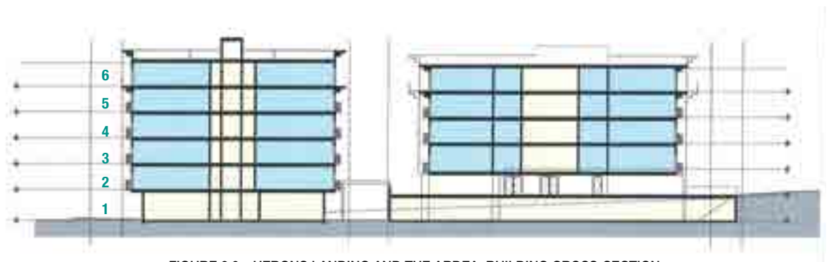
FIGURE 2.6 - HERONS LANDING AND THE ARDEA: BUILDING CROSS-SECTION
