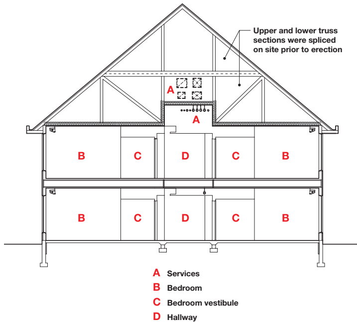
FIGURE 4 Section through a typical home area
