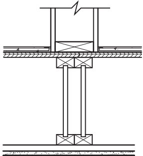
FIGURE 3 Typical Roof, Wall and Floor Sections
