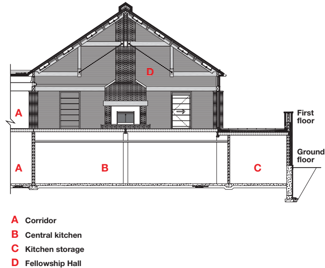
FIGURE 4 Section through Fellowship Hall
