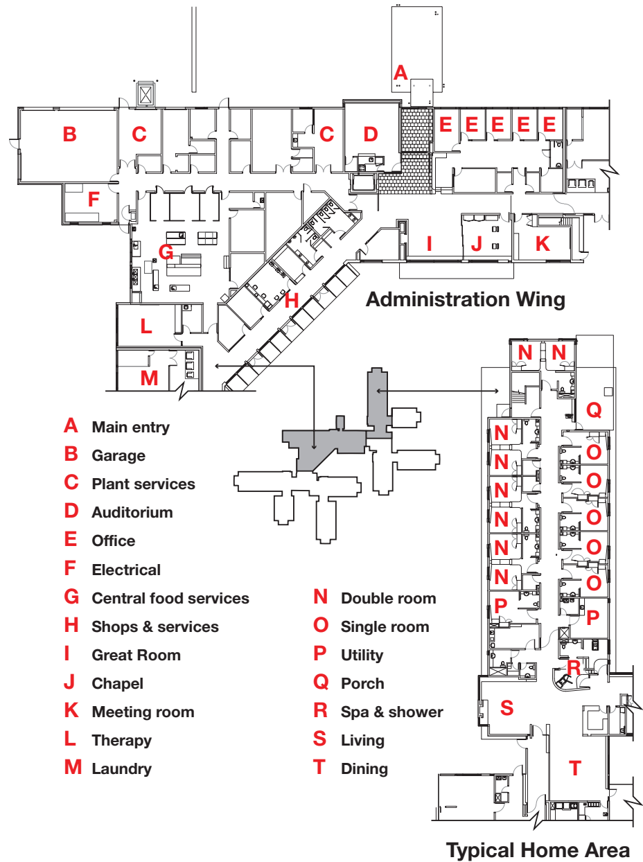
FIGURE 2 Configuration of the central area and a home area
