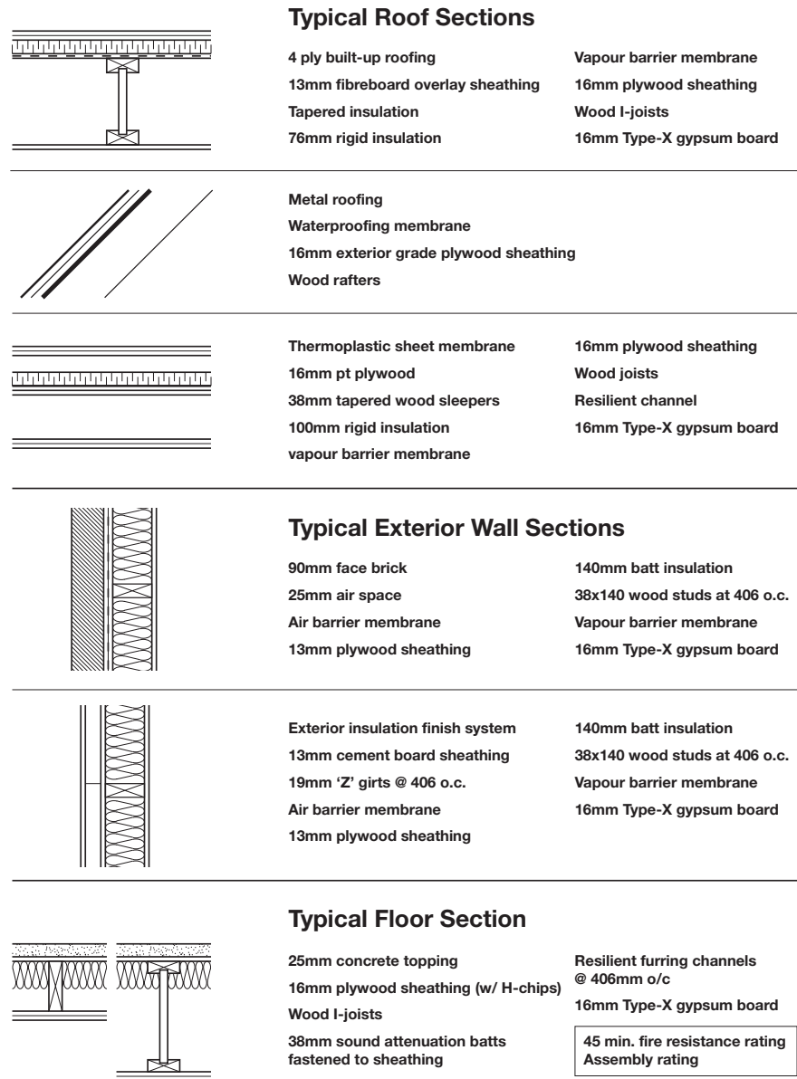
FIGURE 3 Typical Roof, Wall and Floor Sections
