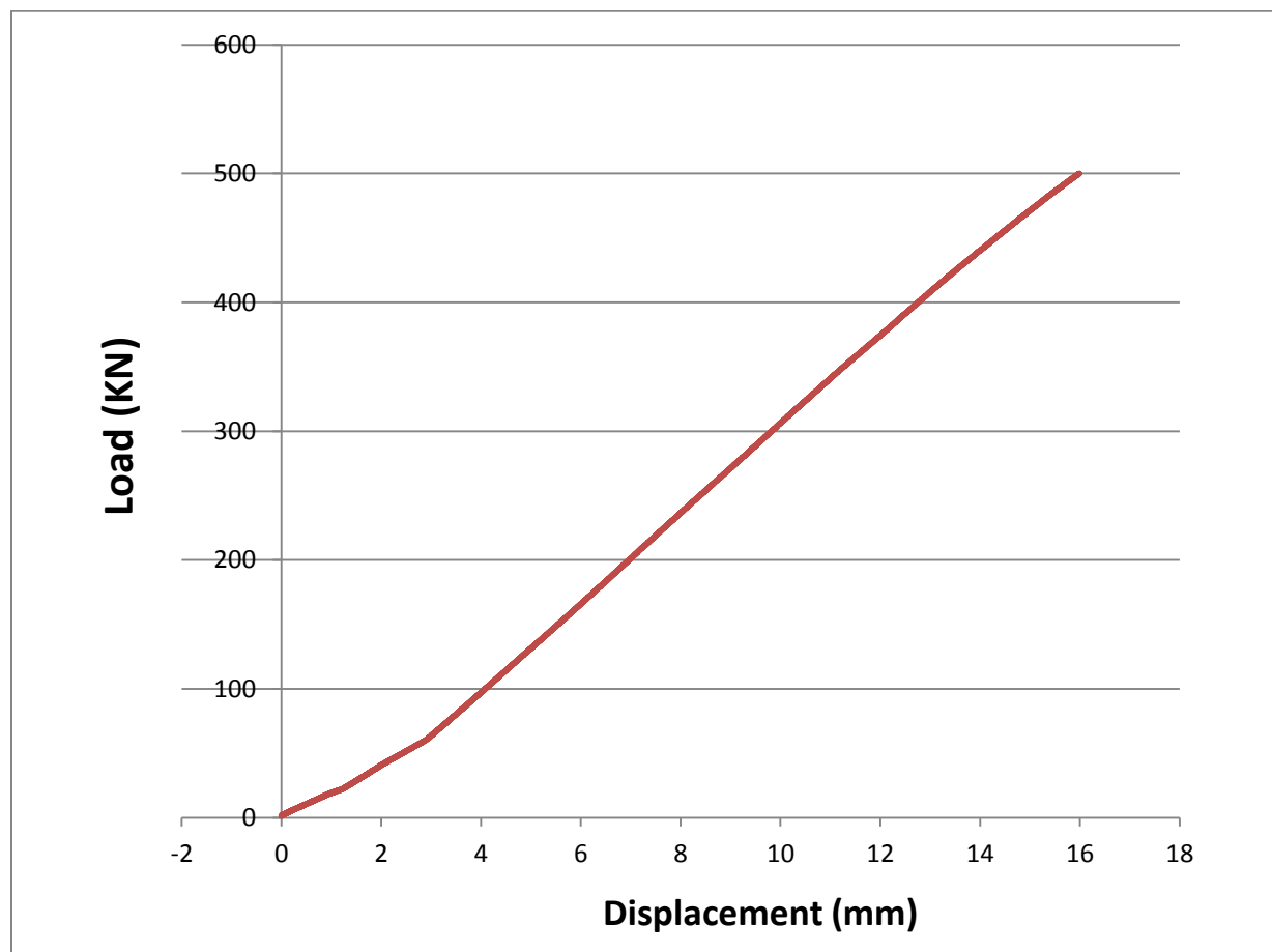
Figure A2. Load-Displacement curve for the CLT specimen 4x12-2
