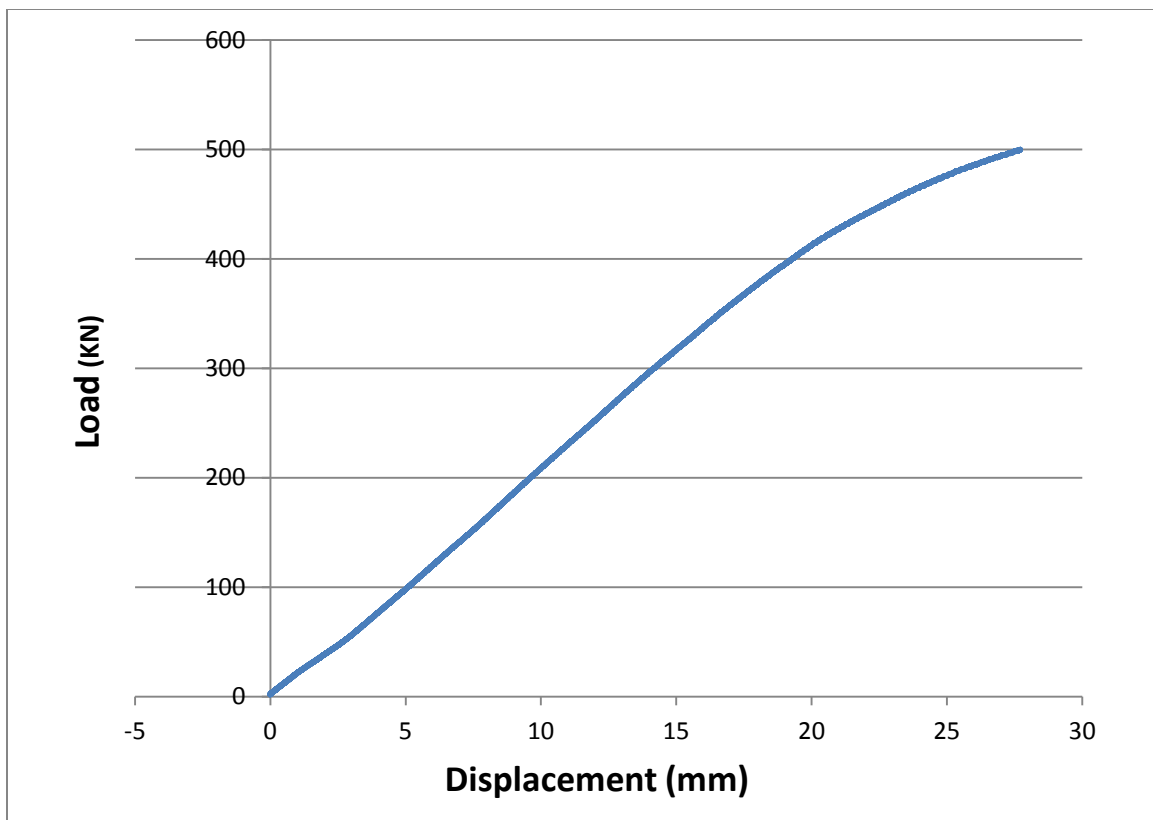
Figure A3. Load-Displacement curve for the specimen 4x20-1
