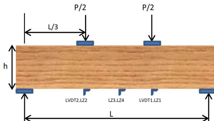
Figure 7. Loading pattern and instrumentation for the 4 feet x 28 feet specimens (Series C)
