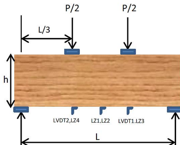
Figure 5. Loading pattern and instrumentation for the 4 feet x 12 feet specimens (Series A)
