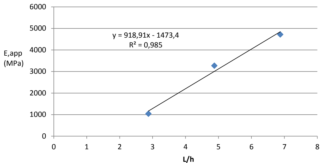
Figure 9. The relationship between the apparent Modulus of Elasticity (E app ) and the span to depth ratio (L/h) for all specimens tested
