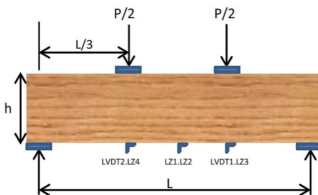
Figure 6. Loading pattern and instrumentation for the 4 feet x 20 feet specimens (Series B)
