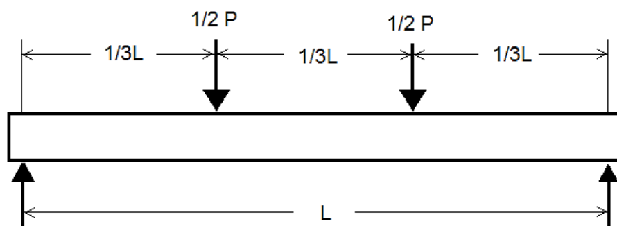
Figure 2. Schematic of the third-point loading setup
