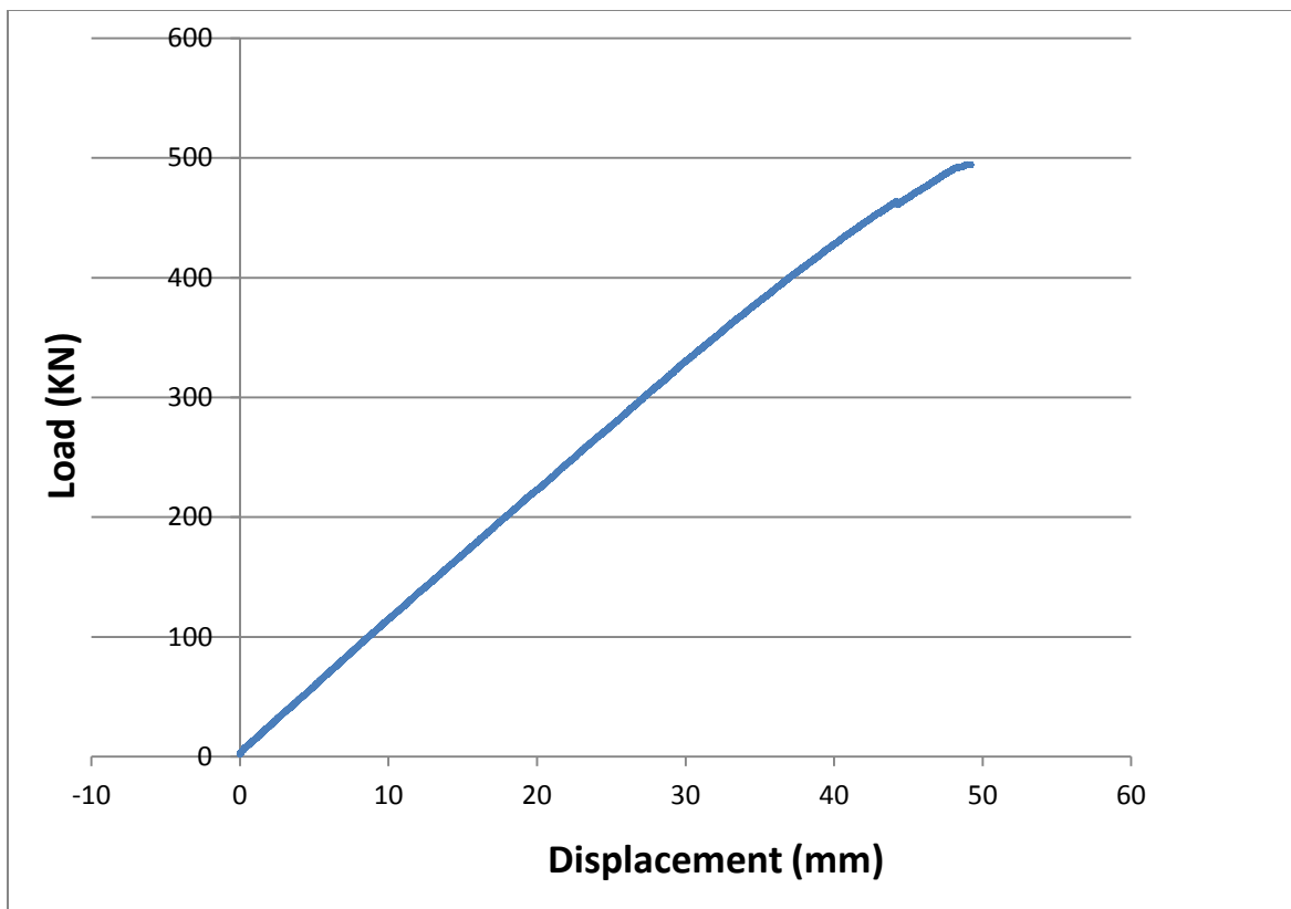
Figure A5. Load-Displacement curve for the specimen 4x28-1
