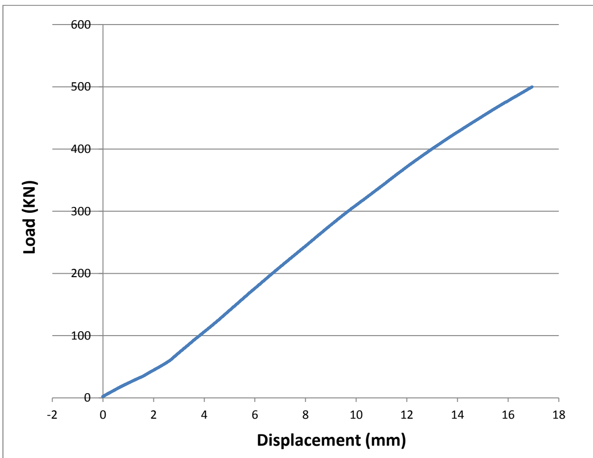
Figure A1. Load-Displacement curve for the CLT specimen 4x12-1
