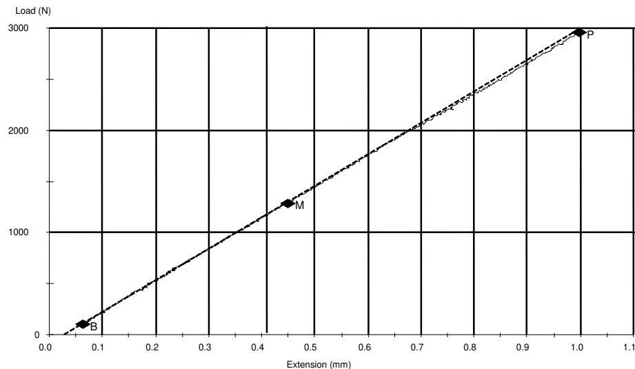
Figure 8. Typical load-deflection curve and determination of the slope
