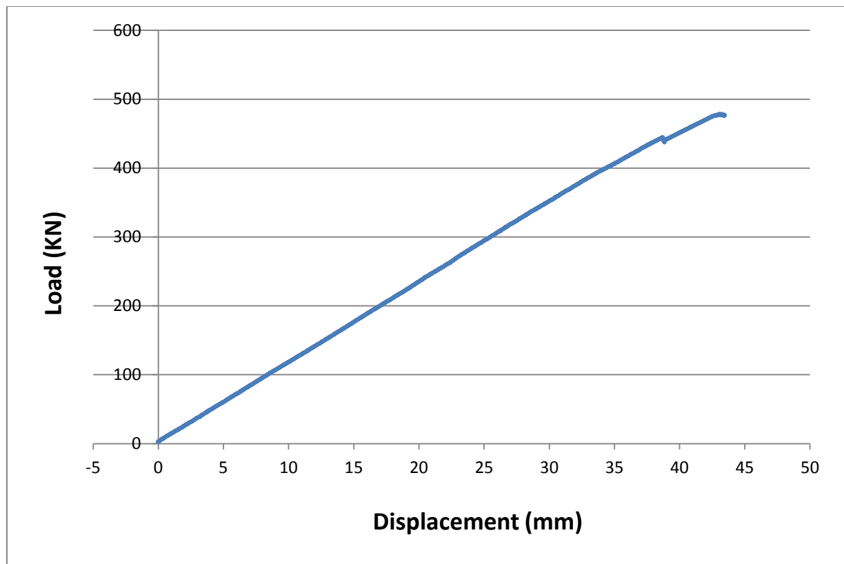
Figure A6. Load-Displacement curve for the specimen 4x28-2
