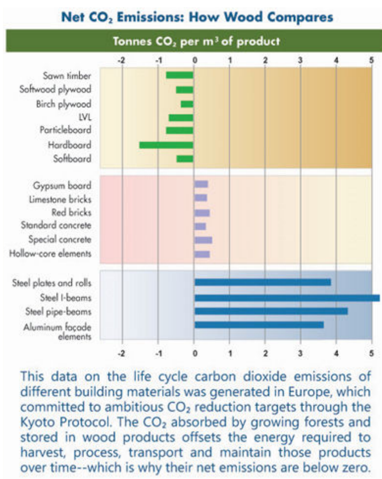
Figure 2.9. Net CO 2 emissions for various construction materials. (Source: https://www.ontario.ca/page/benefits-using-ontario-wood and as noted in the figure).
