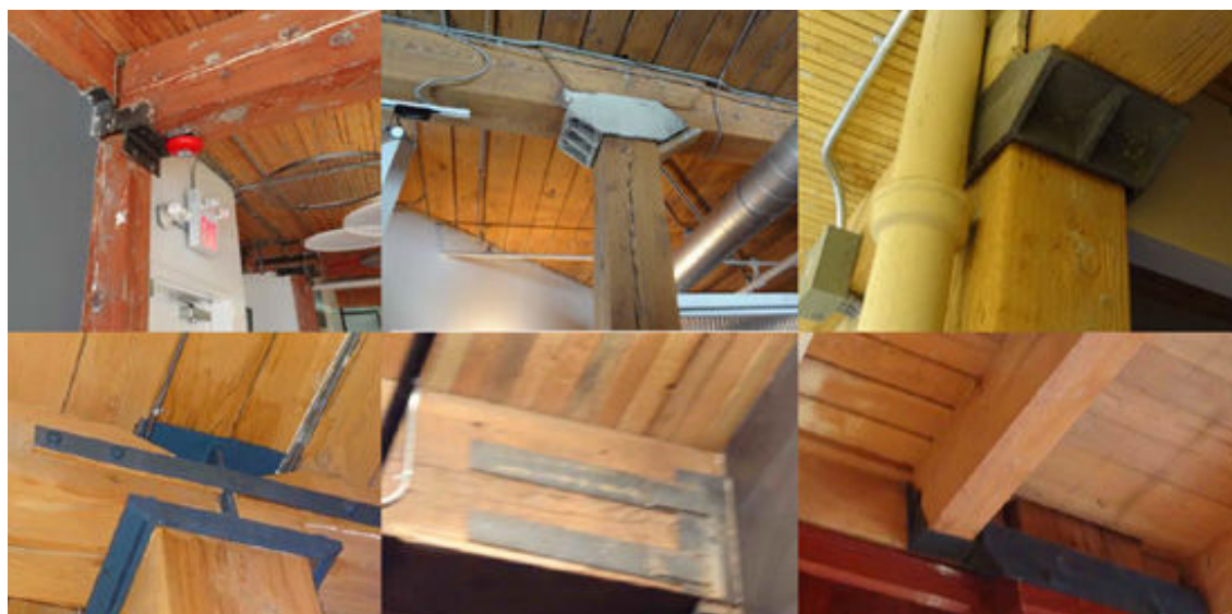
Figure 2.2. Typical historic post and beam connections (from Appendix C-2, Koo, 2013). Metal castings provide end-grain bearing to reduce the effects of wood shrinkage.
