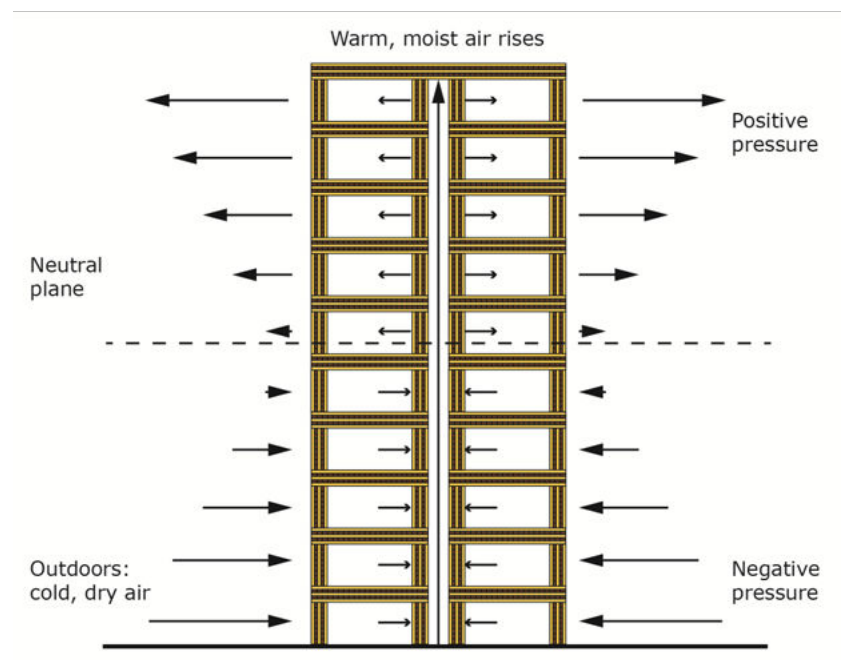
Figure 3.2. Illustration showing stack effect in high-rise building during winter months [From Figure 6 of Chapter 5 from FPInnovations Technical Guide for the Design and Construction of Tall Wood Buildings in Canada].
