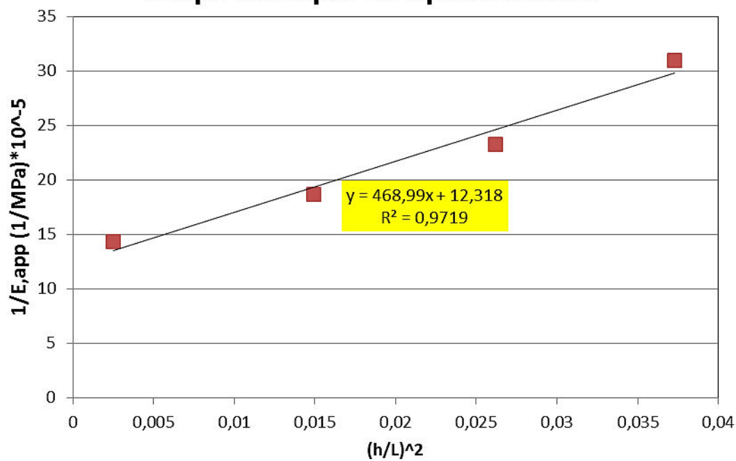
Graph Example for Specimen A 3
