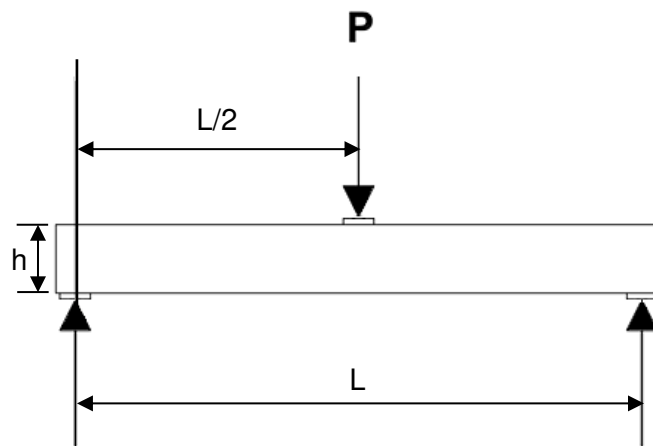
Figure 2. Schematic of Center-point loading setup
