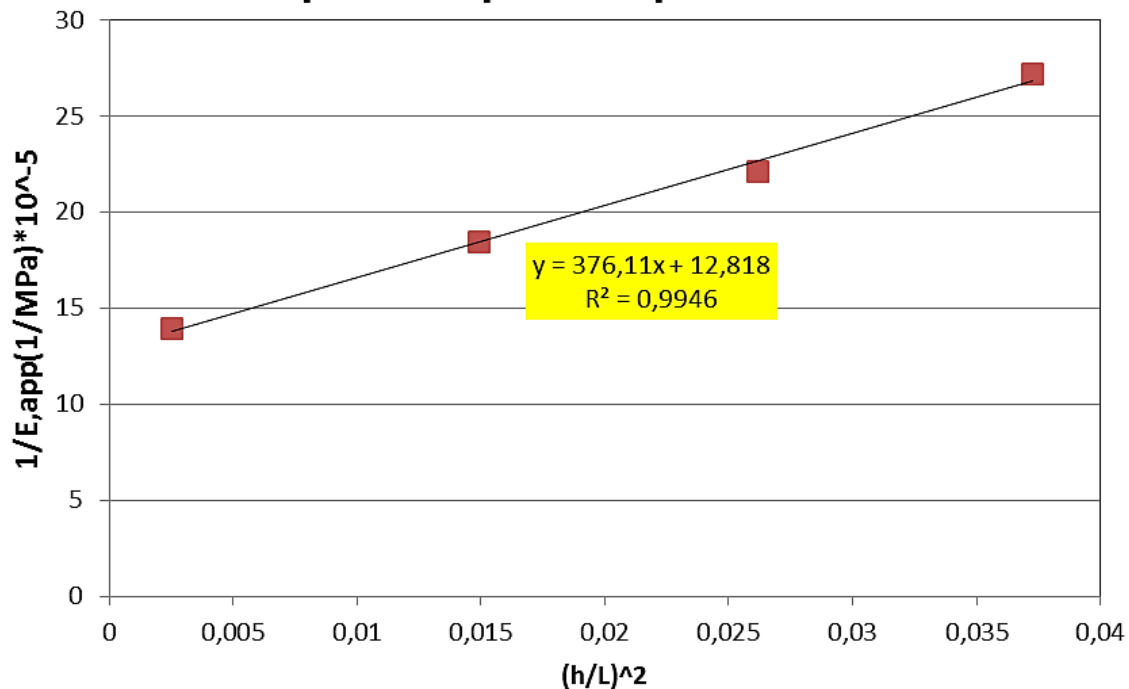
Graph Example for Specimen F 3
