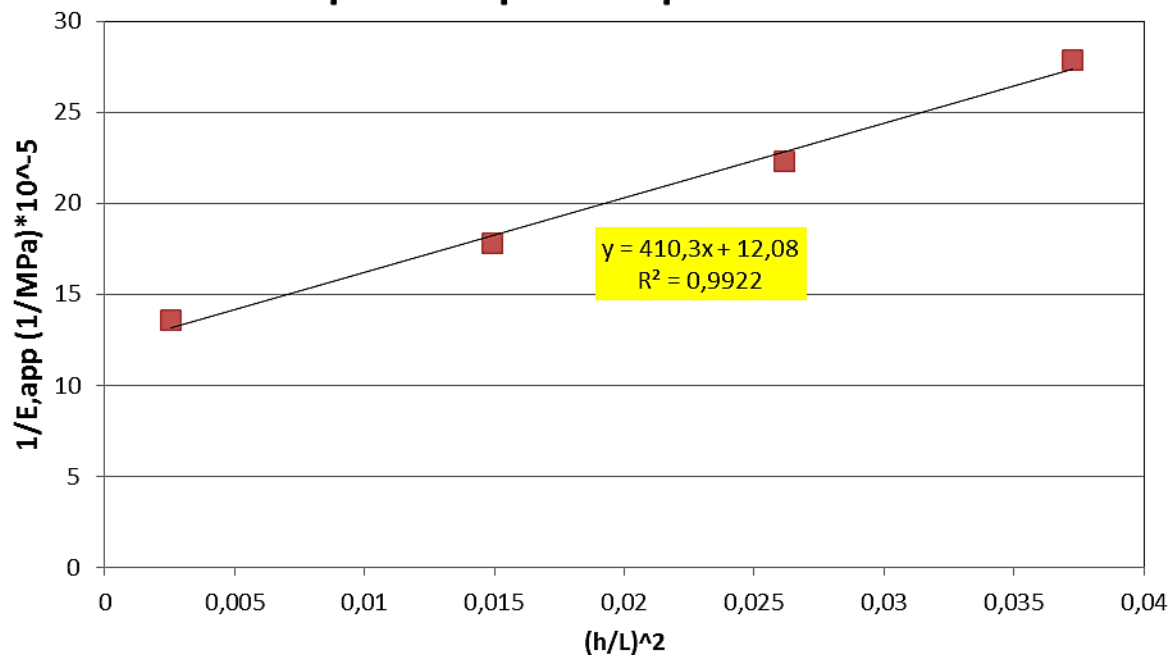
Graph Example for Specimen G 3
