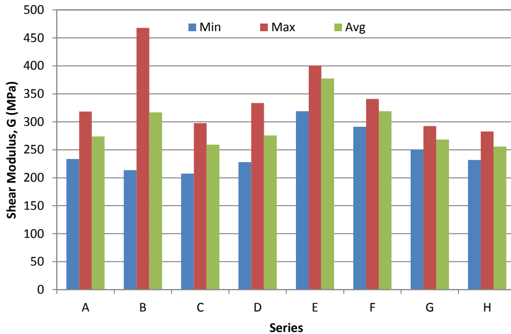
Figure 7. Minimum, Maximum, and Average Shear Moduli
