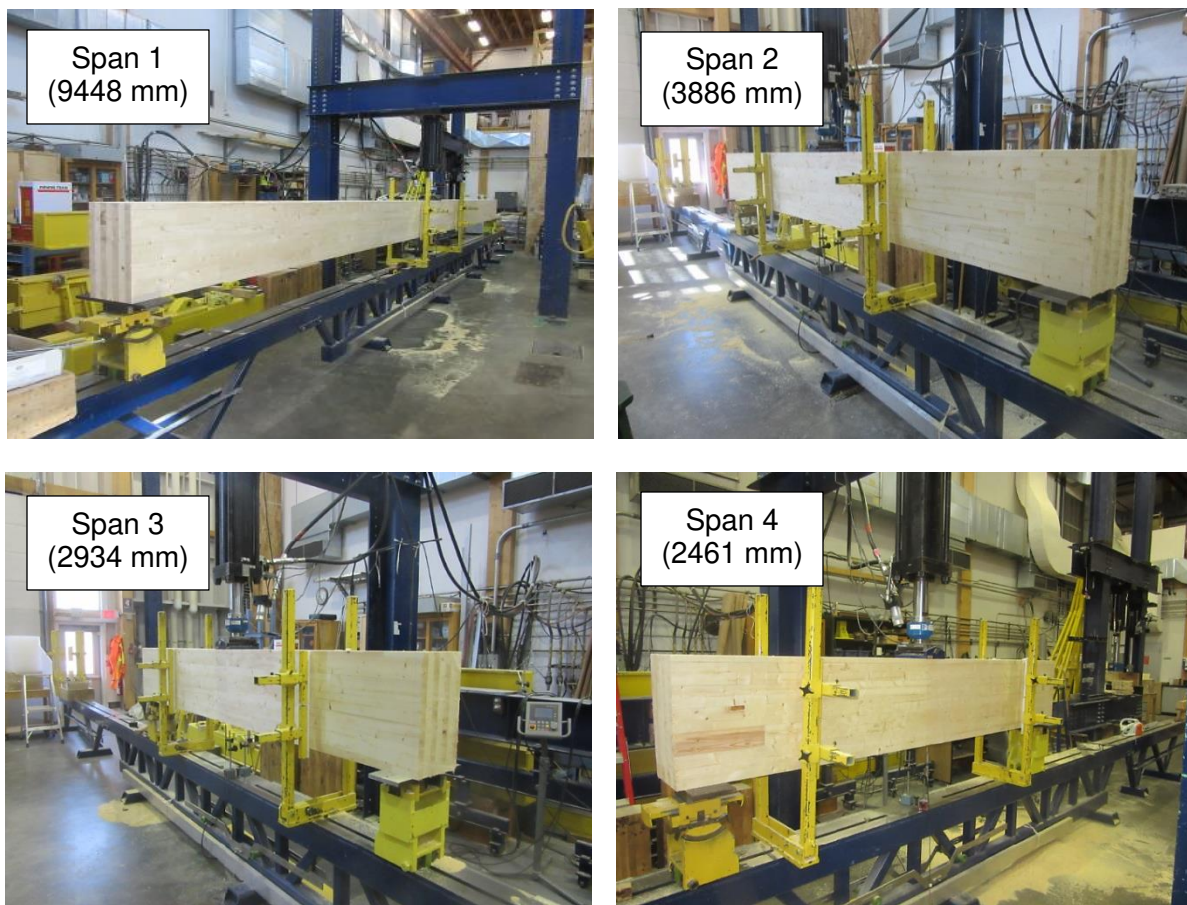
Figure 3. Specimen from Series H tested at the four (4) different spans
