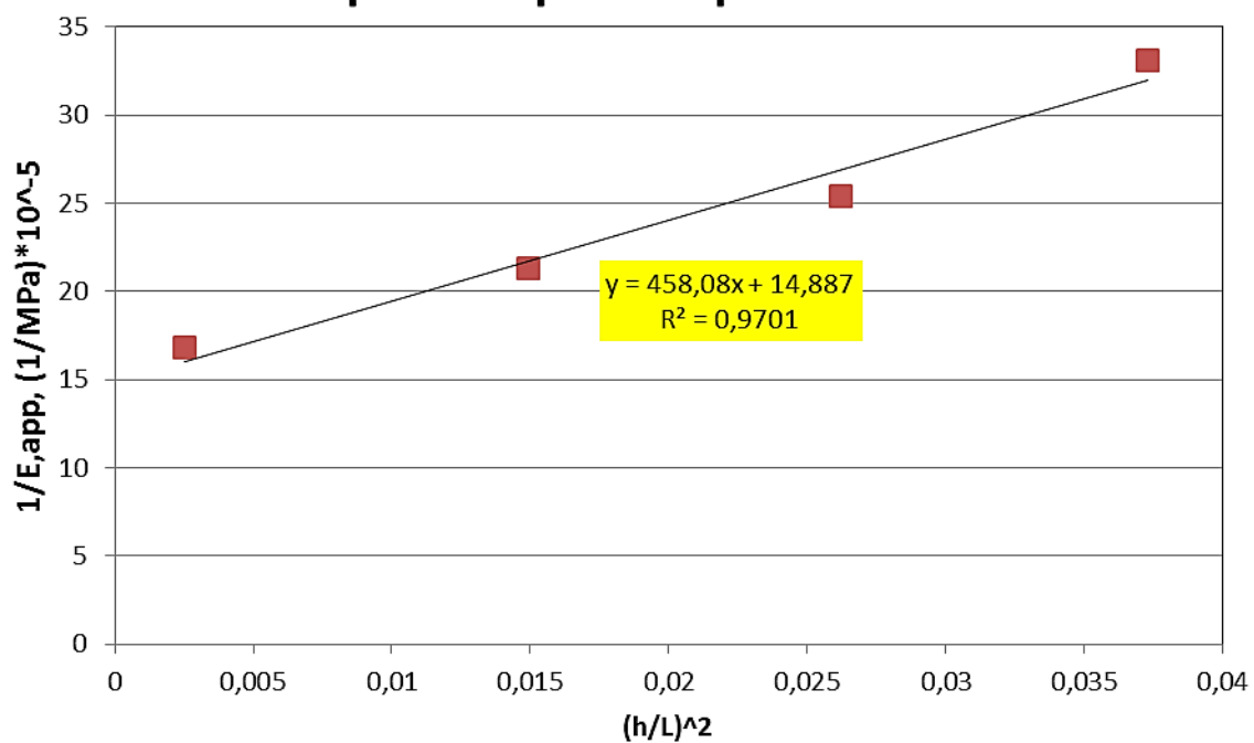
Graph Example for Specimen C 2
