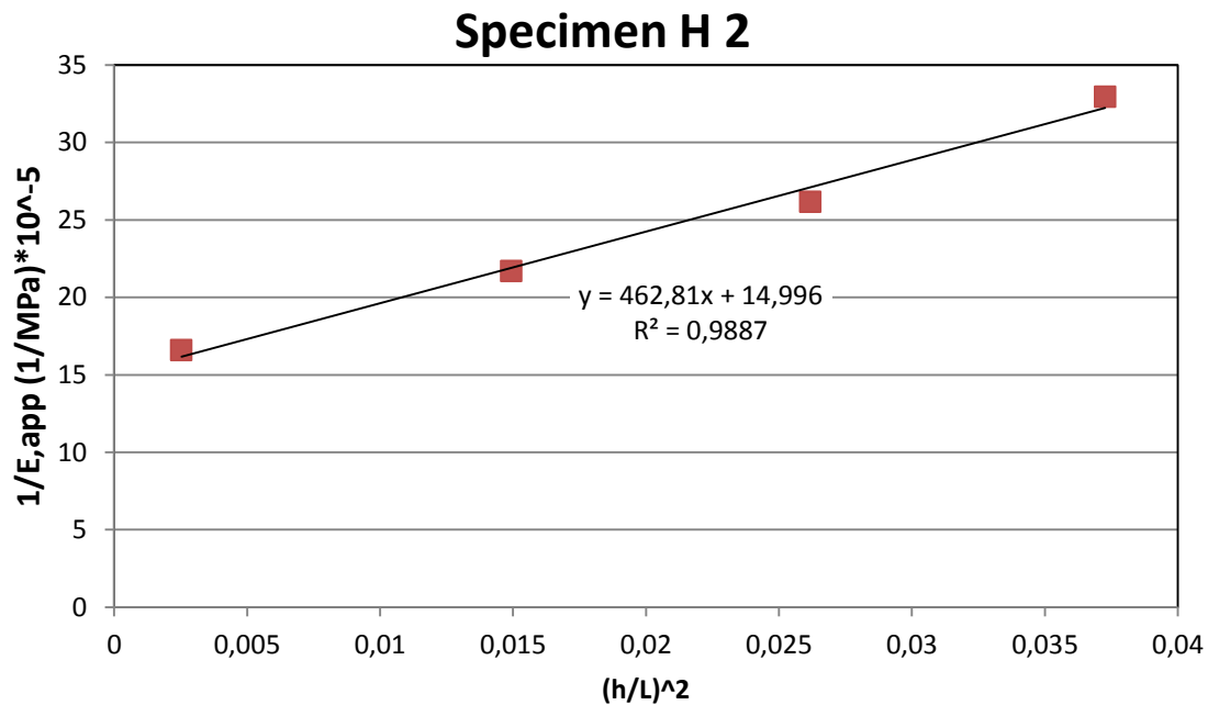
Figure 5. Plot for determination of Shear Modulus for Specimen 2 of Series H
