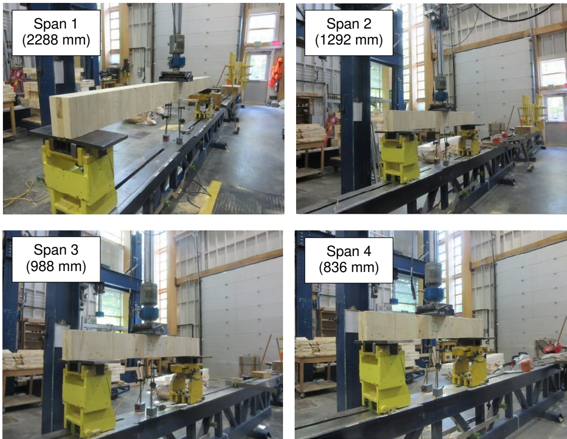
Figure 4. Specimen from Series B tested at the four (4) different spans
