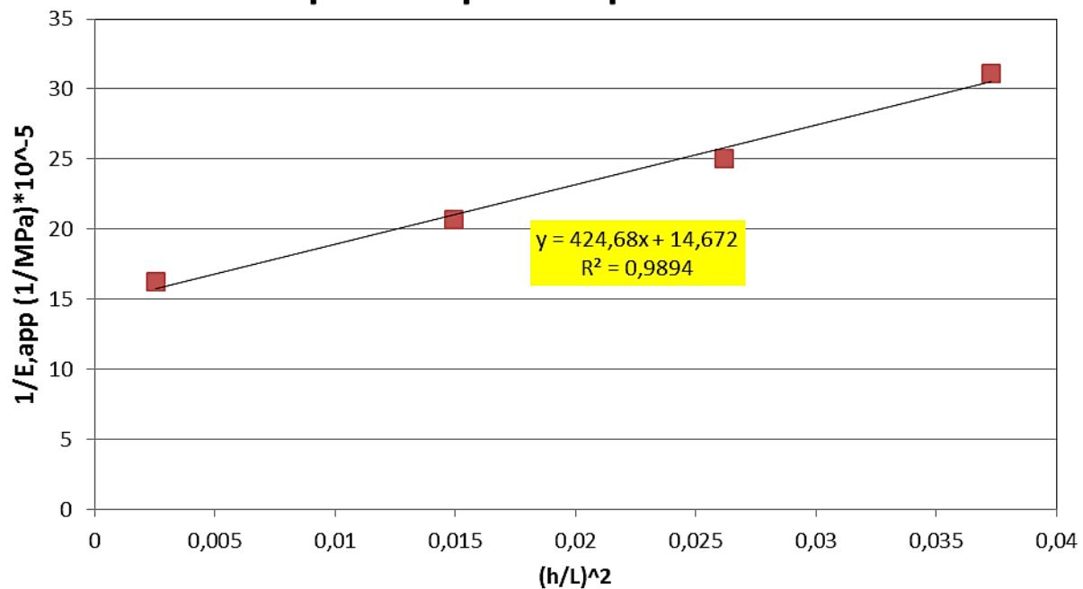
Graph Example for Specimen H 7
