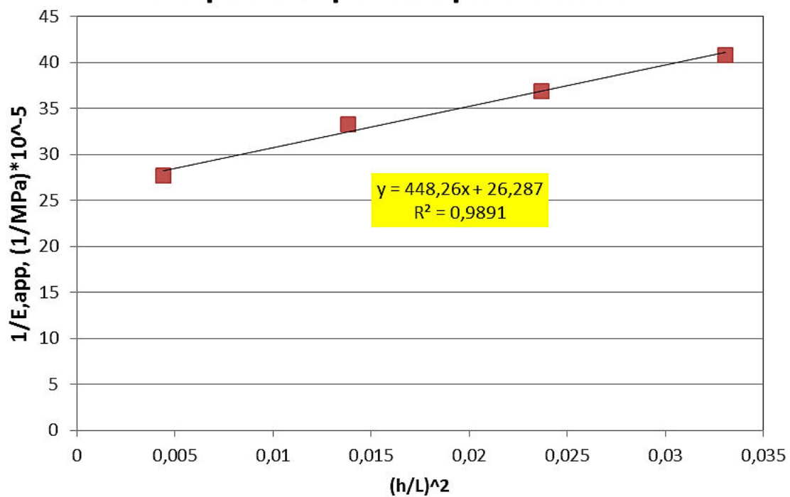
Graph Example for Specimen B 7
