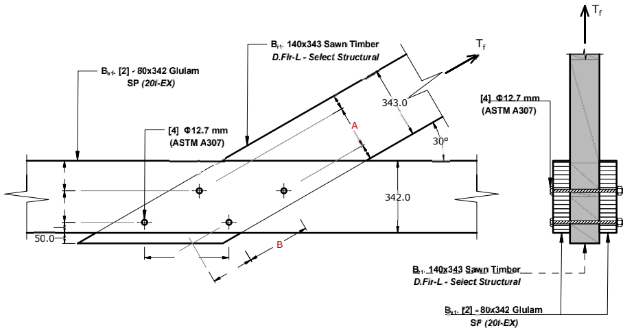
Detail B
