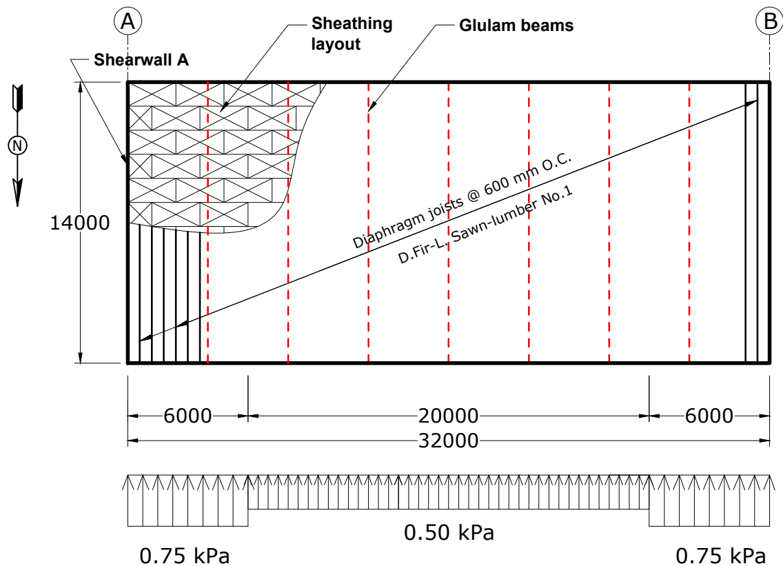
Roof Plan
