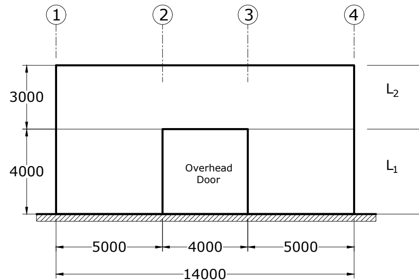
East Elevation
