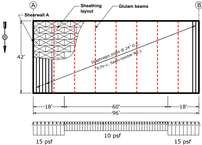
Roof Plan
