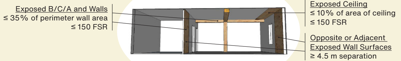
Figure 6 Permitted exposed mass timber within a suite – Option A
