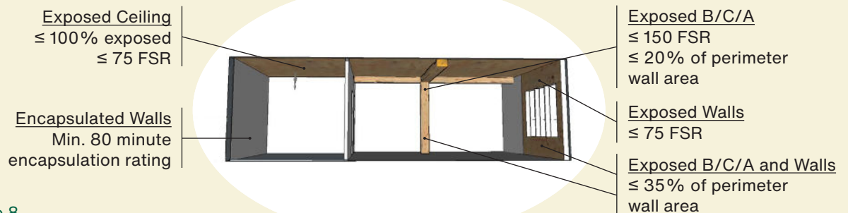
Figure 8 Permitted exposed mass timber within a suite – Option C
