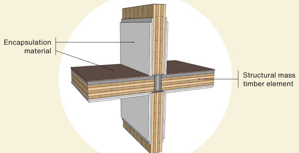
Figure 3 Elements forming encapsulated mass timber construction
