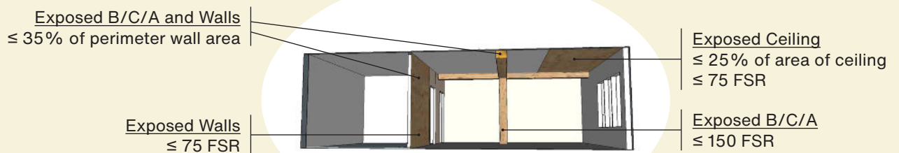
Figure 7 Permitted exposed mass timber within a suite – Option B
