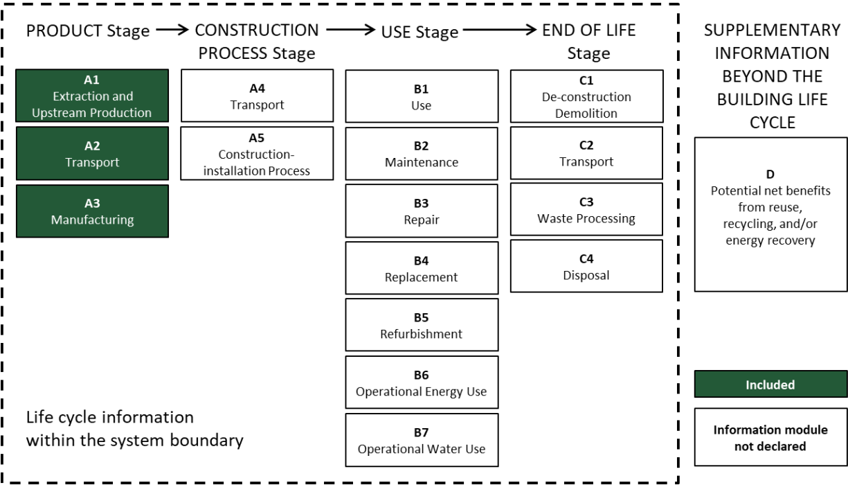
Figure 2: System boundary
